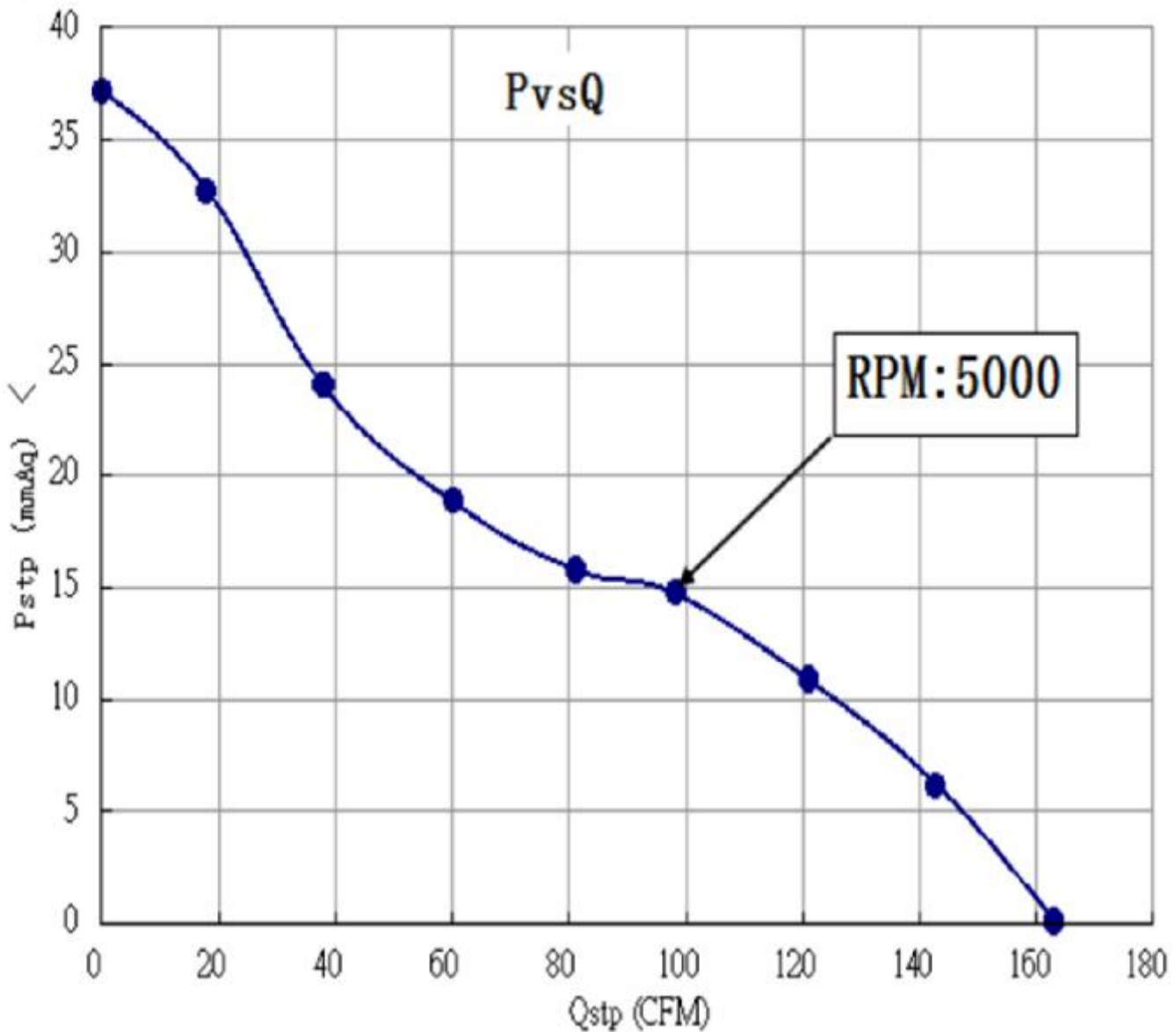
PERFORMANCE CURVES(性能曲线)
