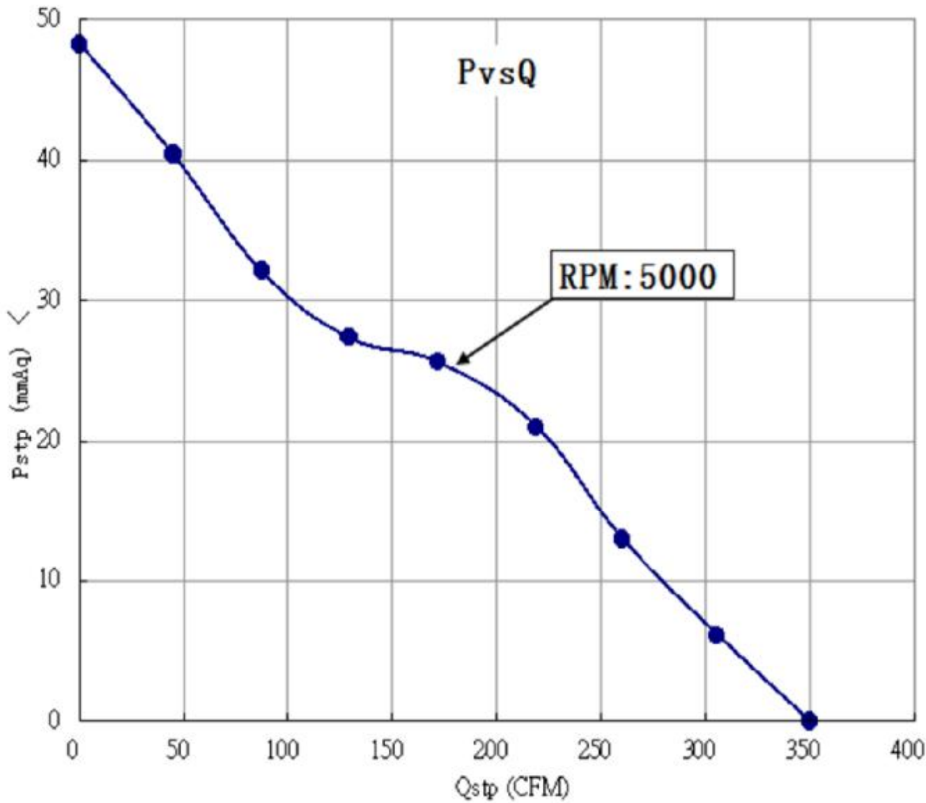
PERFORMANCE CURVES(性能曲线)
